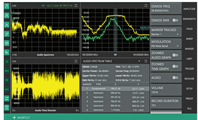
The AM/FM Modulation Measurements Screen Provides a Unique Simultaneous Display of Results and RF and Audio Spectrum
