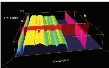
3D Spectrogram For In-Depth Analysis with 3-Axis Rotation Viewing, Threshold, Reference Level, and Marker Control. Turn on Signal ID to See the Types of Signals.
