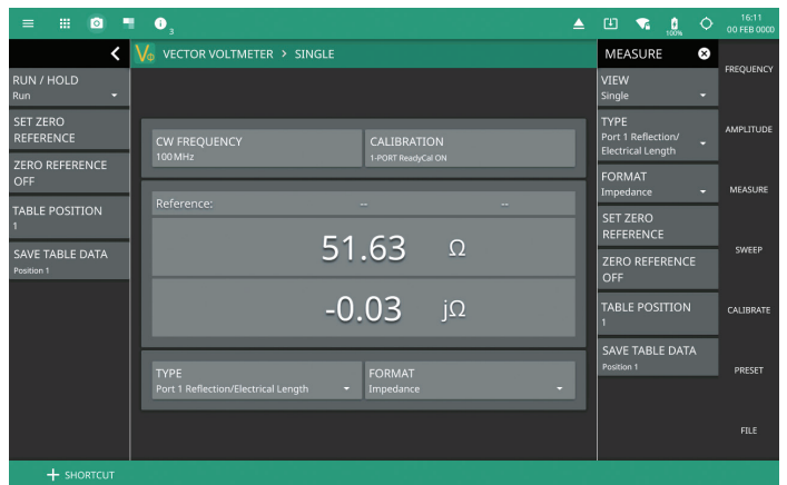
Complex Impedance
