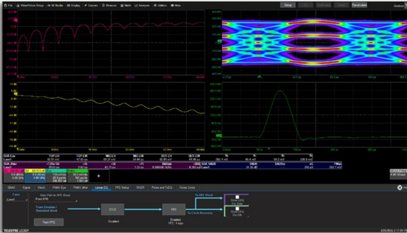
Optimize the equalizer at the receiver and see the impact on the eye diagram.
